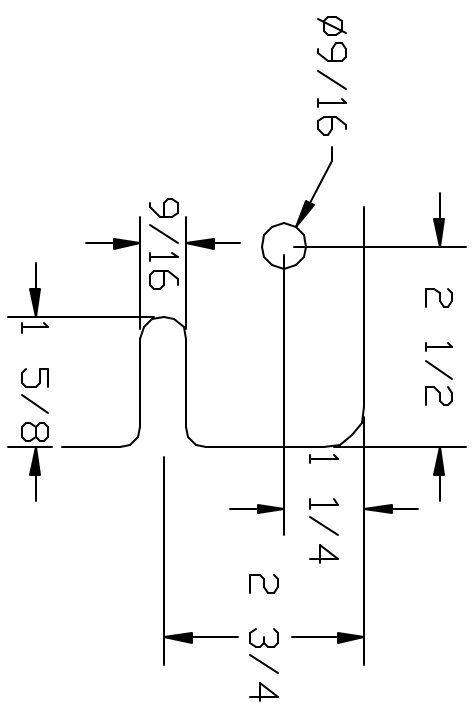
CORNER DETAIL
